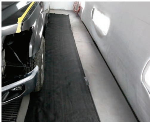
Netting can be used on the booth floor by securing with duct tape. Will trap overspray and dirt from getting in wet paint.
